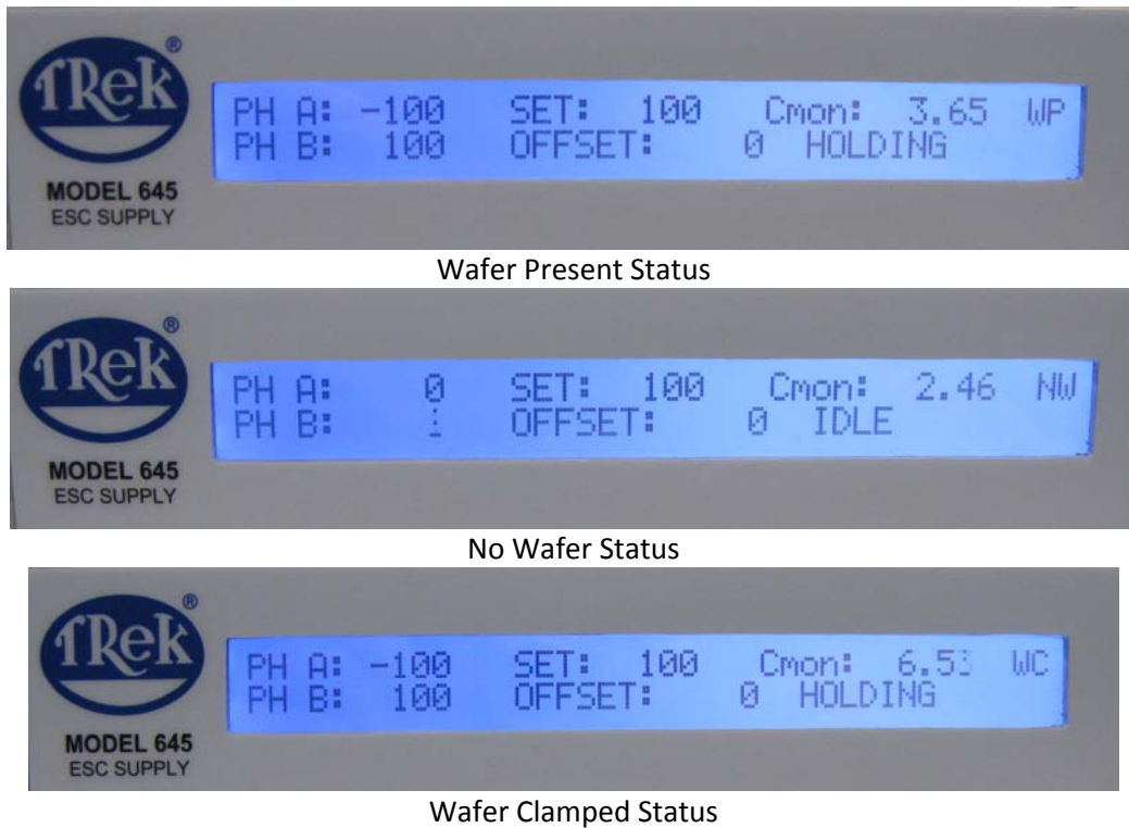
Figure 7. Display of the wafer status on the ESC.
