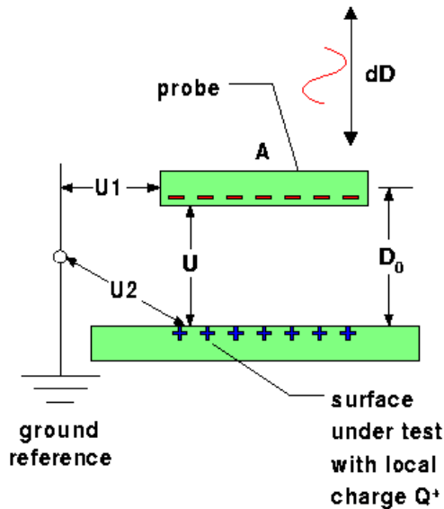
Figure 1: Parallel-plate capacitor.
