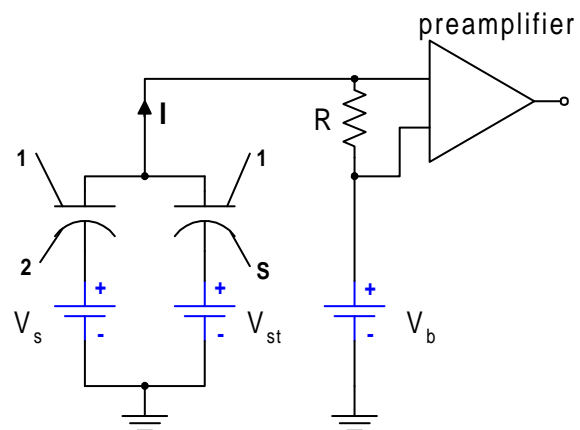
Figure 1: Equivalent circuit for stray capacitance effects.
